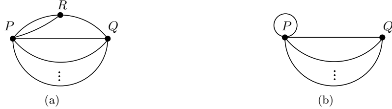
FIGURE 2. (a) \deg(P) = g + 1 , \deg(Q) = g , \deg(R) = 3 .
