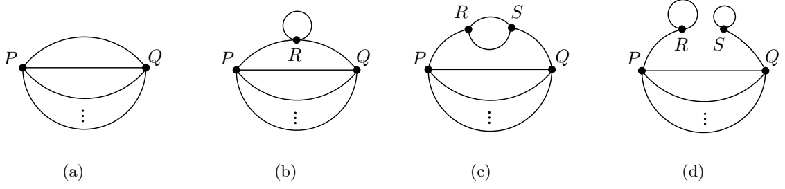
FIGURE 1. Cases where K is not very ample, c.f., Theorem 10.
