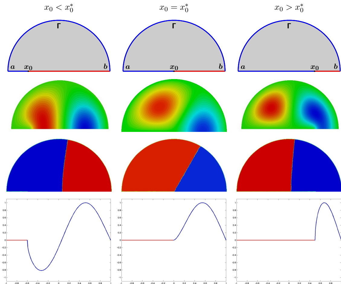
Figure 10: Eigenfunctions for the Dirichlet-Neumann problem on the half-disk. First row: the domain, Second row: the second eigenfunction \varphi_{x_0} , Third row: the nodal domains of \varphi_{x_0} , Fourth row: trace of \varphi_{x_0} on y = 0 .
