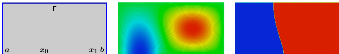
Figure 14: Eigenmodes for the Neumann-Dirichlet-Neumann problem on the half-square. Left: the domain, Center: the second eigenfunction, Right: the associated nodal domains.
