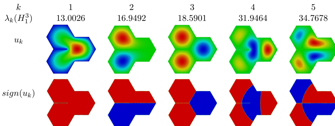
Figure 19: First five eigenmodes on cracked 3-hexagons H_1^3 .
