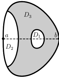
Figure 3: The 3-partition has one circle and one line.
