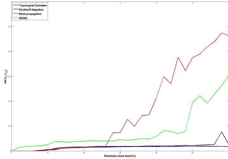
Fig. 1.4. Standard deviations of localization error with respect to electronic noise level for \mathcal{I}_{\text{MU}} , \mathcal{I}_{\text{BP}} , \mathcal{I}_{\text{KM}} , and \mathcal{I}_{\text{TD}} with n = 50 .
