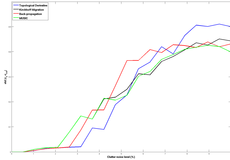
Fig. 1.11. Standard deviations of the localization error with respect to clutter noise for \mathcal{I}_{\text{MU}} , \mathcal{I}_{\text{BP}} , \mathcal{I}_{\text{KM}} , and \mathcal{I}_{\text{TD}} with n = 50 .
