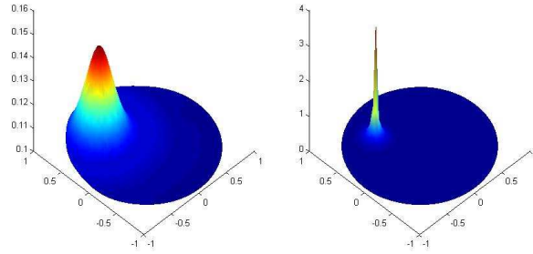
Fig. 1.2. Left: MUSIC image using the projection of \mathbf{g}^{(1)}, \mathbf{g}^{(2)} , and \mathbf{g}^{(3)} on the signal subspace of \mathbf{A} . Right: MUSIC image using the projection of \mathbf{g}^{(3)} on the signal subspace of \mathbf{A} .
