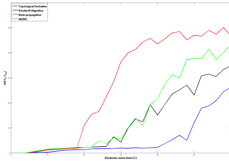
Fig. 1.10. Standard deviations of localization error with respect to electronic noise level for \mathcal{I}_{\text{MU}} , \mathcal{I}_{\text{BP}} , \mathcal{I}_{\text{KM}} , and \mathcal{I}_{\text{TD}} with n = 50 .
