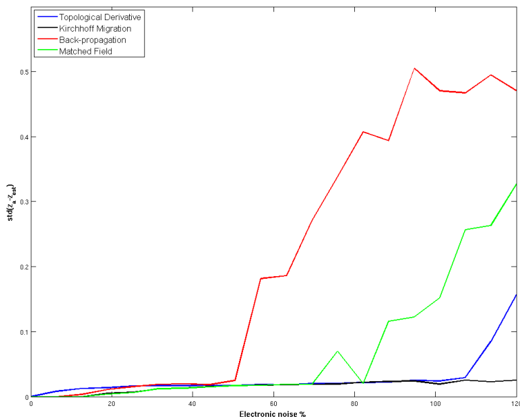
Fig. 1.12. Standard deviations of the localization error with respect to measurement noise for \mathcal{I}_{\text{BPF}} , \mathcal{I}_{\text{KMF}} , \mathcal{I}_{\text{MF}} , and \mathcal{I}_{\text{TDF}} with m = 30 and n = 50 .
