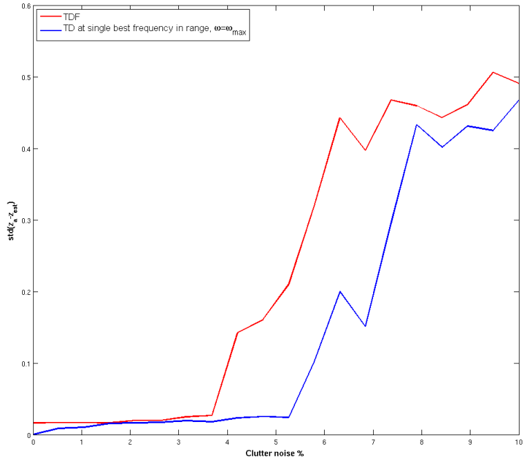
Fig. 1.13. Standard deviations of the localization error with respect to medium noise for \mathcal{I}_{\text{TDF}} with m = 30 and n = 50 and \mathcal{I}_{\text{TD}} at \omega_{\text{max}} for n = 50 .
