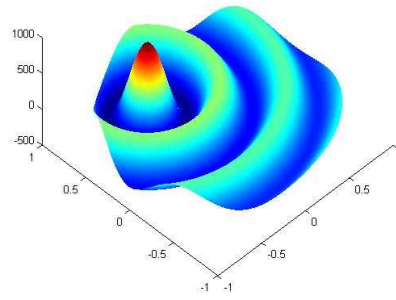
Fig. 1.9. Backpropagation image.
