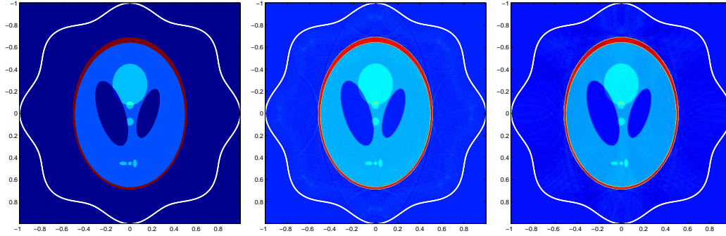
FIGURE 1. Comparison between \mathcal{I}_1 and \mathcal{I}_2 without attenuation a = 0 . Left: source f(x) ; Middle: reconstruction using \mathcal{I}_1 ; Right: reconstruction using \mathcal{I}_2 .
