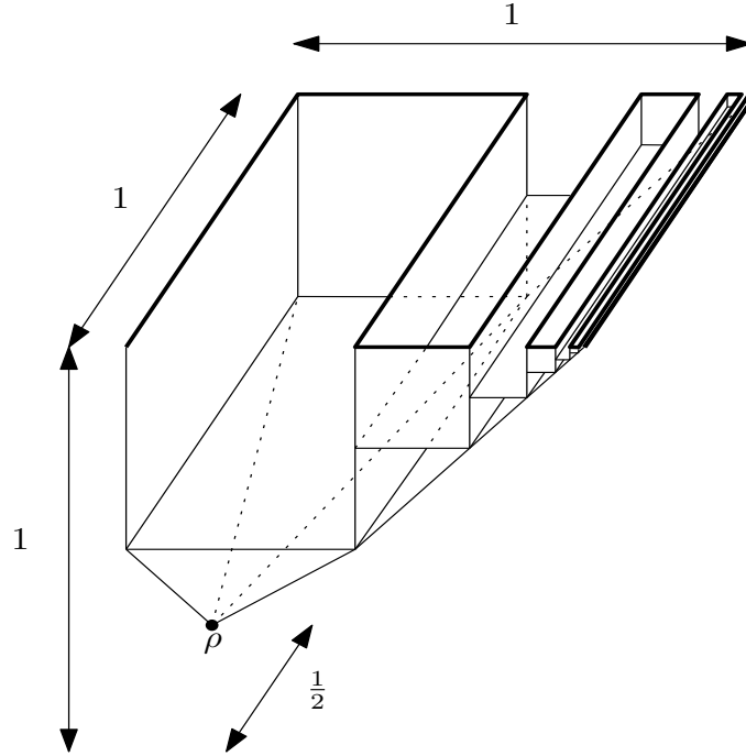
Figure 2: An example of a geodesic compact metric space E , such that the complement of the open ball of radius 1 centered at the distinguished point \rho is connected but not path-connected. Here E is a compact subset of \mathbb{R}^3 and is equipped with the intrinsic distance associated with the L^\infty -metric \delta((x_1, x_2, x_3), (y_1, y_2, y_3)) = \sup\{|x_i - y_i|, i = 1, 2, 3\} . For this distance, the sphere of radius 1 centered at \rho , which coincides with the complement of the open ball of radius 1, consists of the closure of the union of the bold lines at the top of the figure. It is not path-connected, by the same argument as the one showing that the closure of the graph of the function x \mapsto \sin(1/x) on (0, \infty) is a subset of the plane which is not path-connected.
