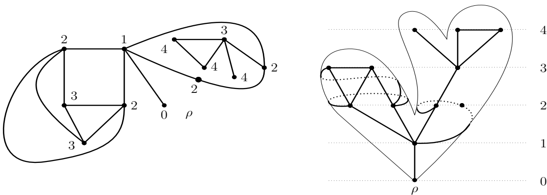
Figure 1: A planar map and on the right side the same planar map represented so that the height of every vertex coincides with its distance from the distinguished vertex \rho . We see a tree structure emerging from this picture, which corresponds to the associated cactus.
