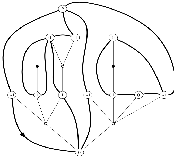
Figure 3: A mobile (\tau, (\ell_u)_{u \in \tau(1,2)}) in \mathbb{T}_+ and its image m under the BDG bijection. Vertices of type 1 are represented by big circles, vertices of type 2 by lozanges, vertices of type 3 by small circles and vertices of type 4 by small black disks. The edges of the tree \tau are represented by thin lines, and the edges of the planar map m by thick curves. In order to get the planar map m one needs to erase the vertices of type 2 and, for each of these vertices, to merge its two incident edges into a single one. The root edge is at the bottom left.
