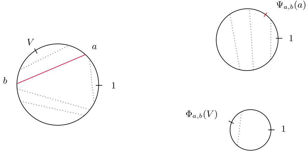
FIG 4. Illustration of the proof in the case V \in R'' .
