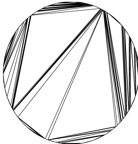
FIG 1. The random set L_\infty .
