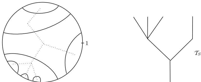
FIG 2. A figela and its associated plane tree (in dotted lines on the left side). We drew chords as curved lines for better visibility. In this example, S has 7 chords and 8 fragments. Notice that each fragment of S corresponds to a vertex of the tree \mathcal{T}_S .
