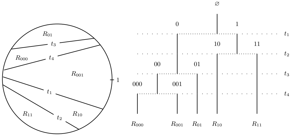
FIG 5. Chords are represented on the left side with their respective creation times. On the right side the genealogical tree of the fragments R_{000}, \dots, R_{11} present at time t_4 .
