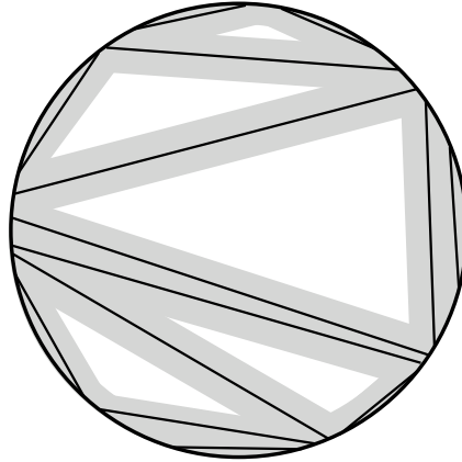
FIG 6. Illustration of the proof of lemma 7.1: The chords [x_i y_i] have to lie in the shaded part of the figure.
