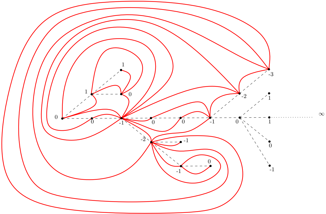
Figure 1: Illustration of the Schaeffer correspondence. The tree is represented in dotted lines and the quadrangulation in solid lines.
