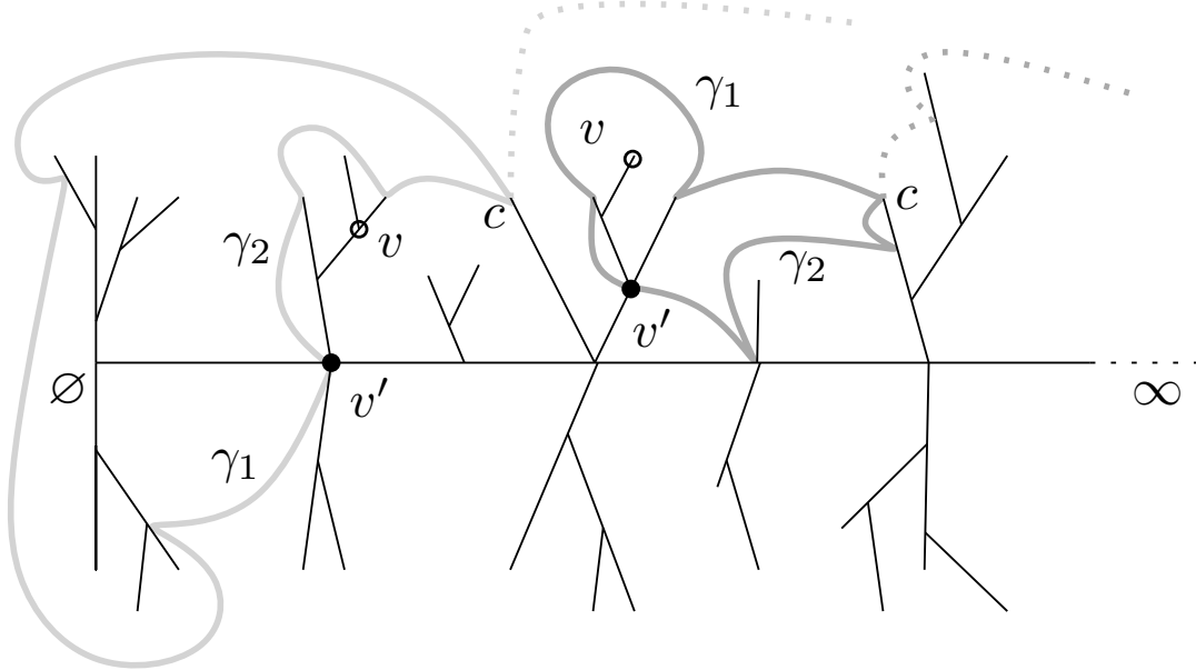
Figure 11: Cycles separating vertices from \emptyset composed by two geodesics.
