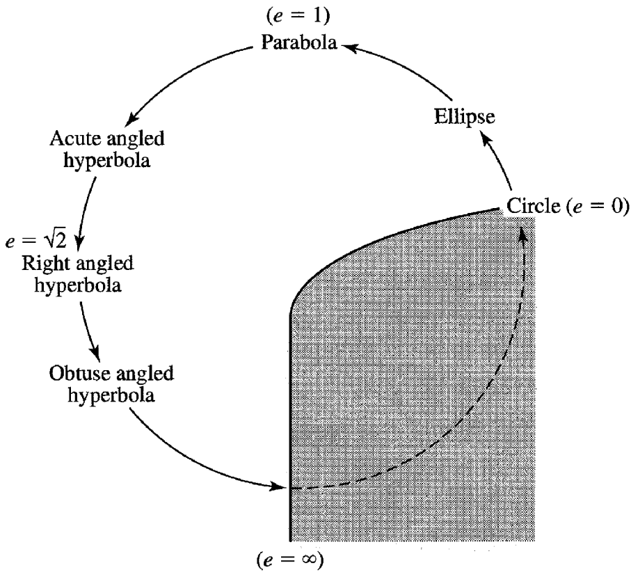
Figure 1.3: Transmigration of a conic
