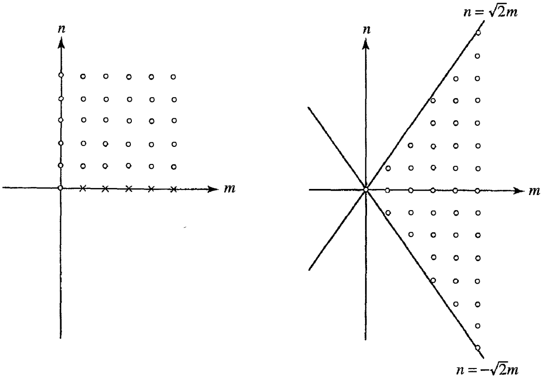
Figure 2.1: Two examples of infinitely generated rings
