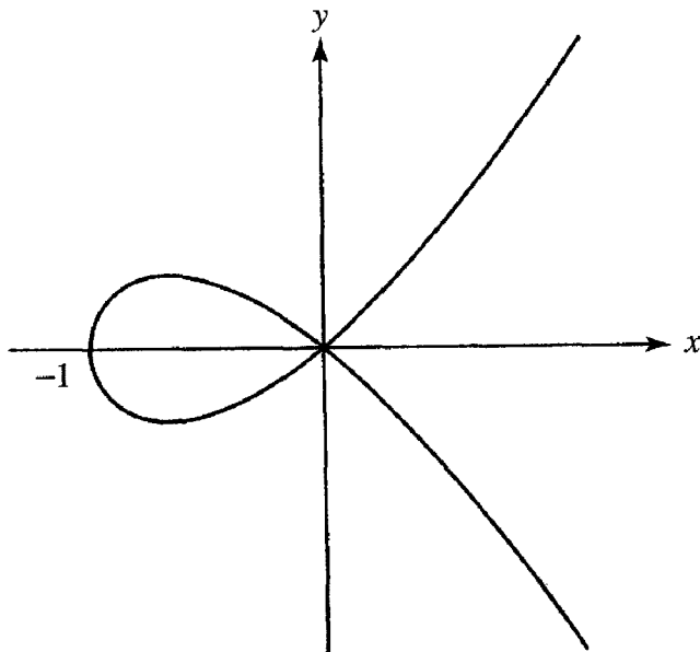
Figure 1.10: The affine plane curve y^2 - x^2 - x^3 = 0
