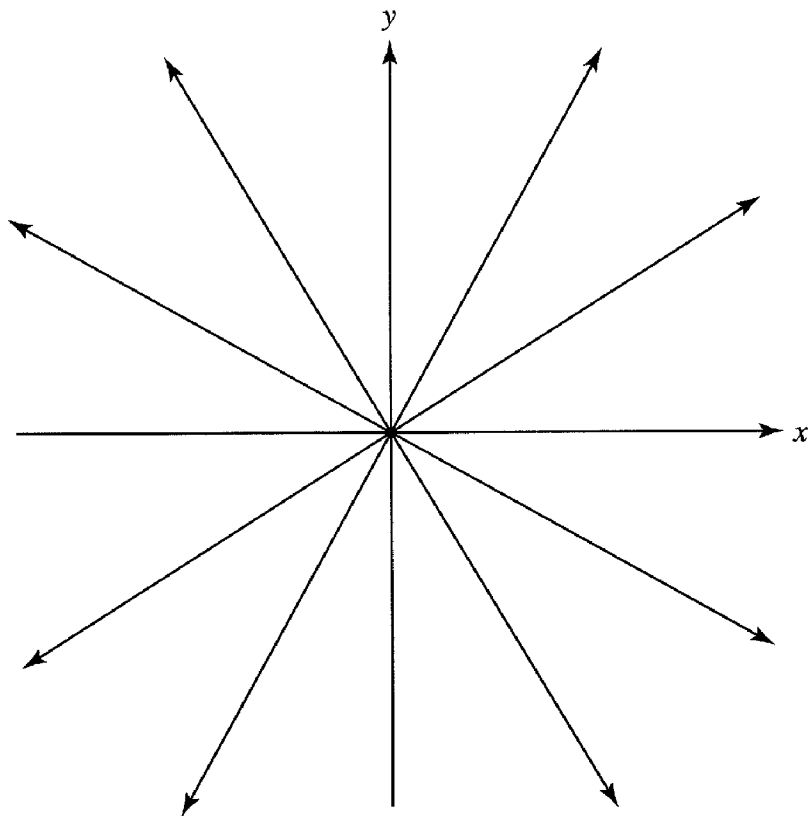
Figure 6.1: The orbits in Example 6.3 ( n = 1 )
