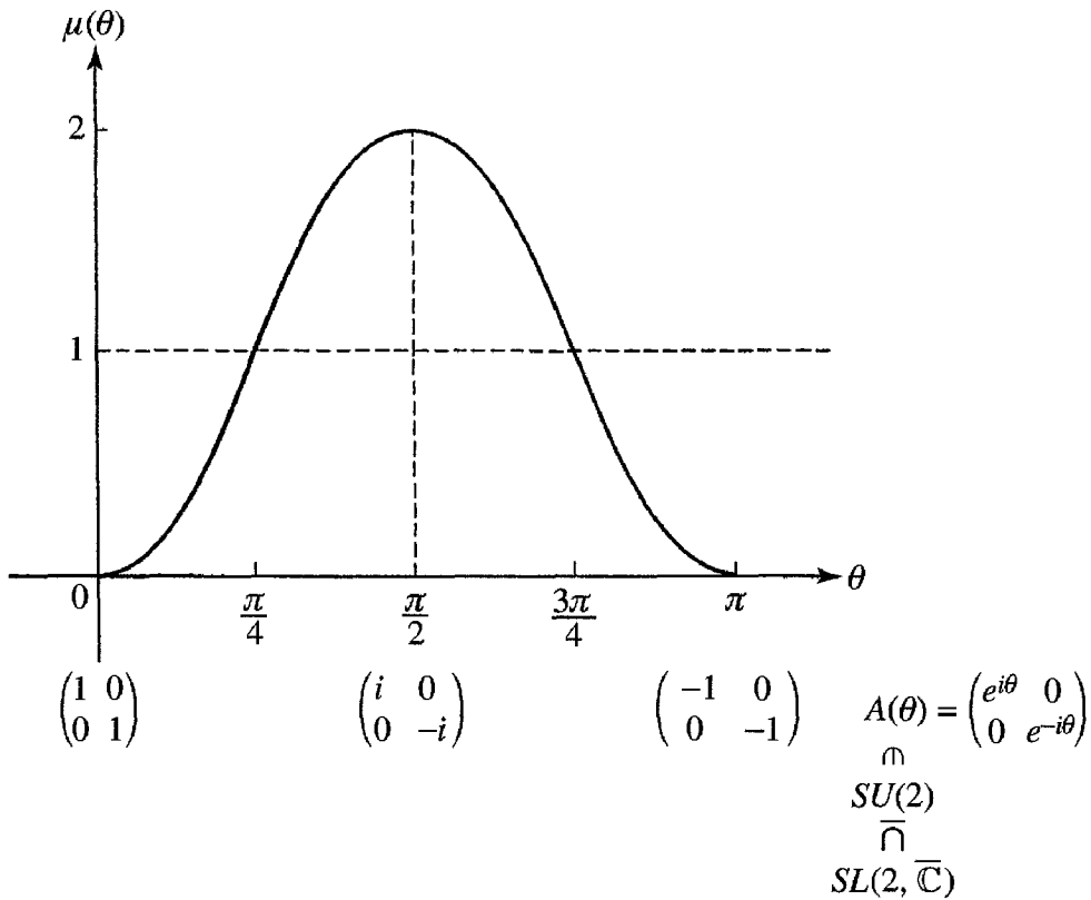
Figure 4.1: Weyl measure \mu(\theta) = 2 \sin^2 \theta
