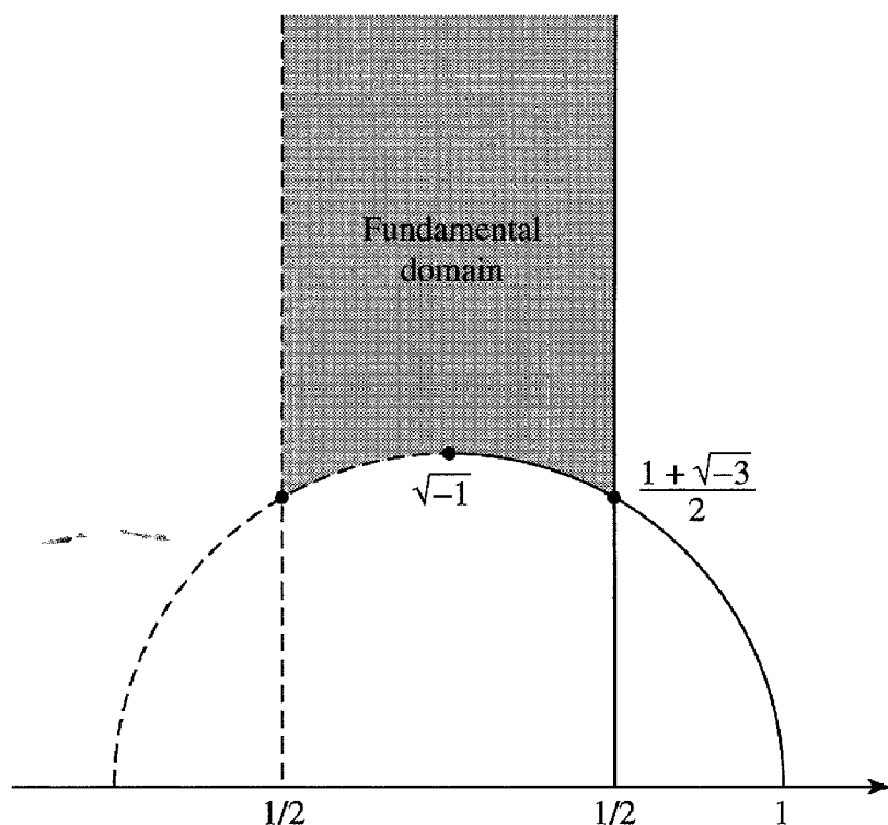
Figure 8.1: The fundamental domain
