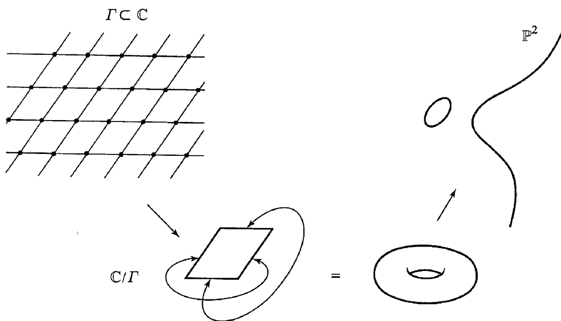
Figure 1.16: A complex cubic curve
