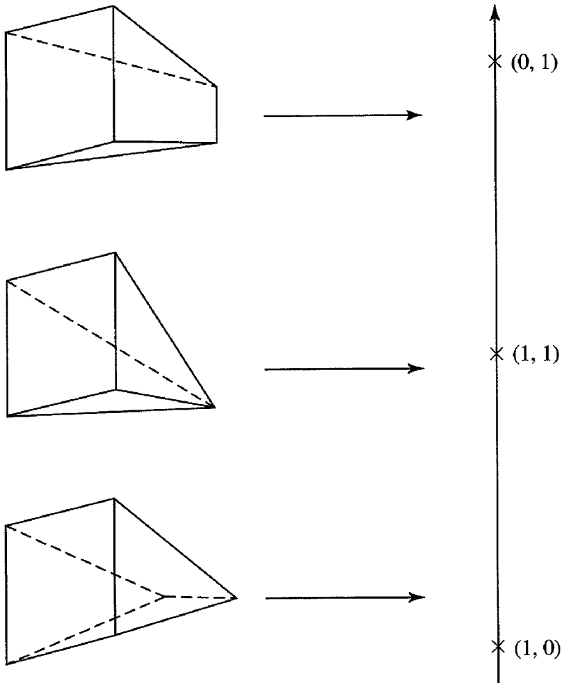
Figure 6.3: Wall crossing
