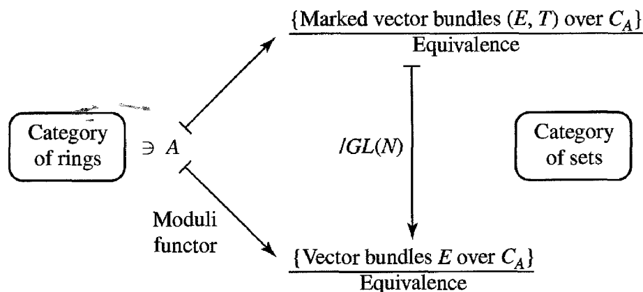
Figure 11.2: The moduli functor for vector bundles
