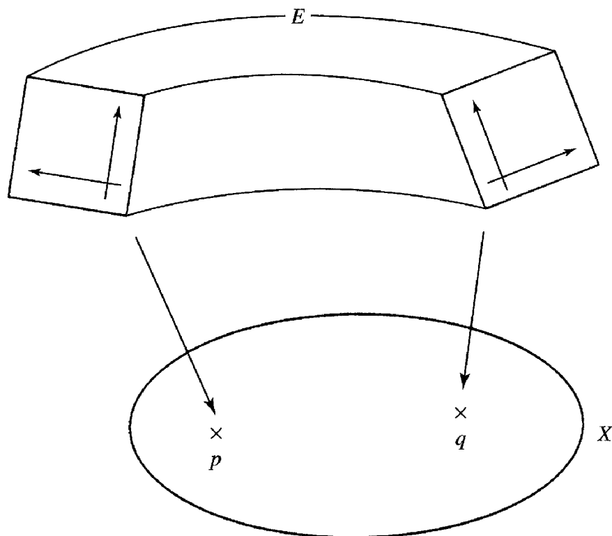
Figure 8.2: A vector bundle E
