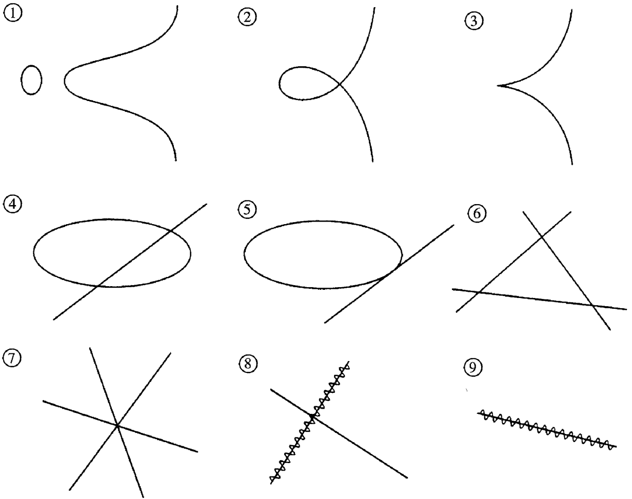
Figure 7.1: Classification of plane cubics
