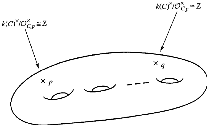
Figure 9.3: Multiplicative principal parts and divisors
