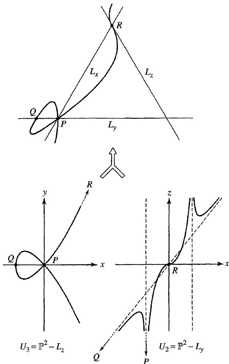
Figure 1.11: The projective plane curve y^2z - x^2z - x^3 = 0
