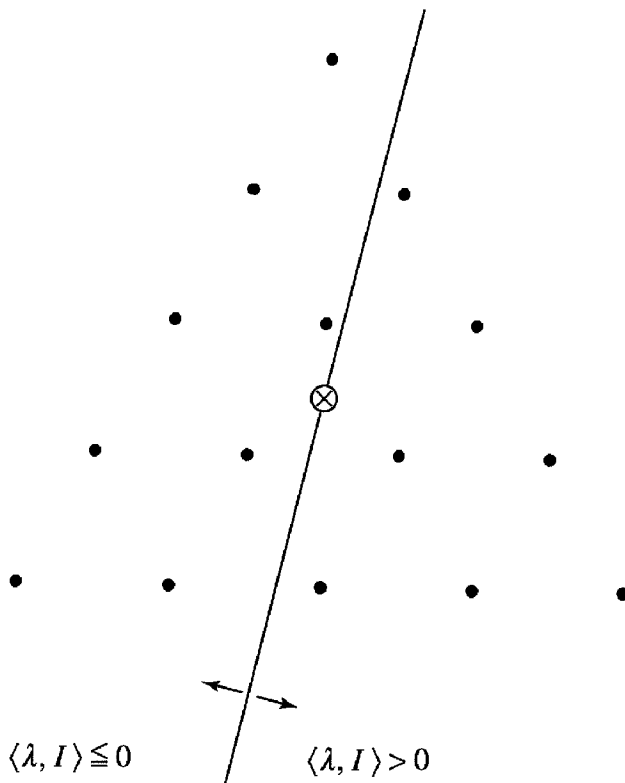
Figure 7.2: Stability of plane quartics
