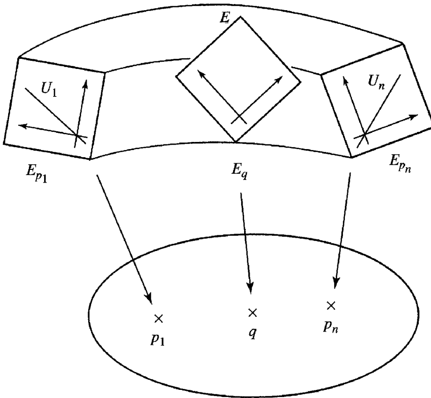
Figure 12.2: A rank 2 quasiparabolic vector bundle
