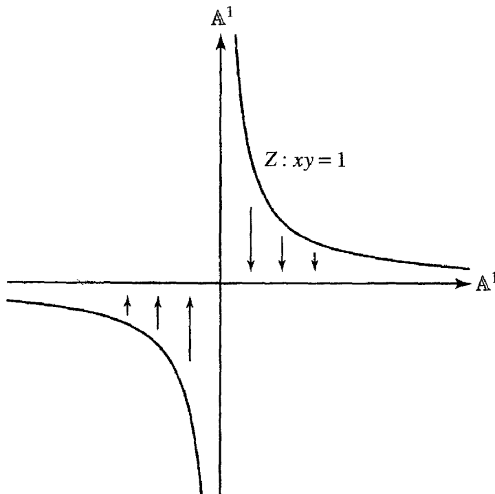
Figure 3.5: The affine line is not complete
