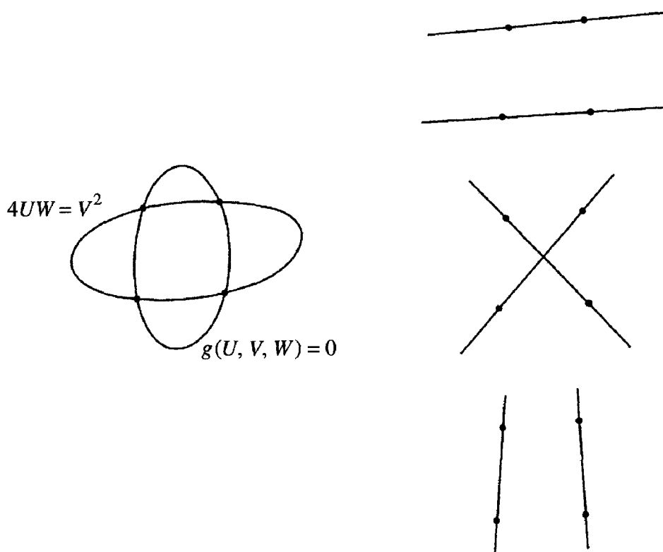
Figure 1.8: Reducible elements in the pencil of conics
