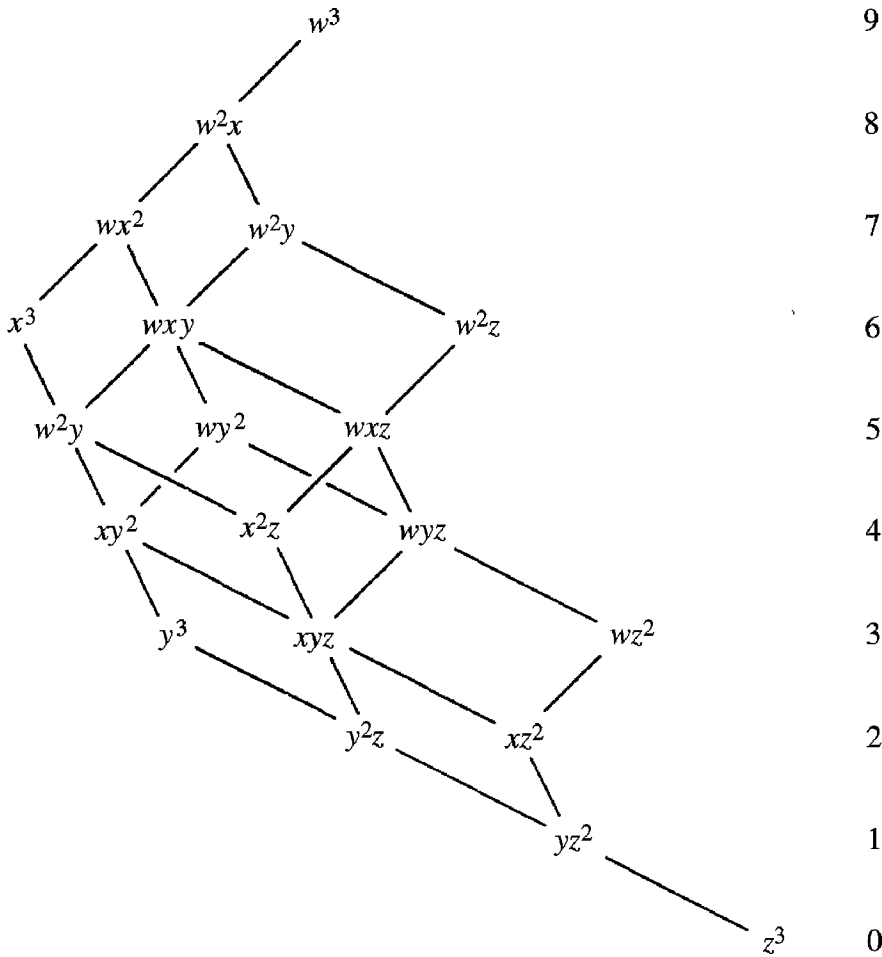
Figure 7.3: Partial ordering of the monomial set M
