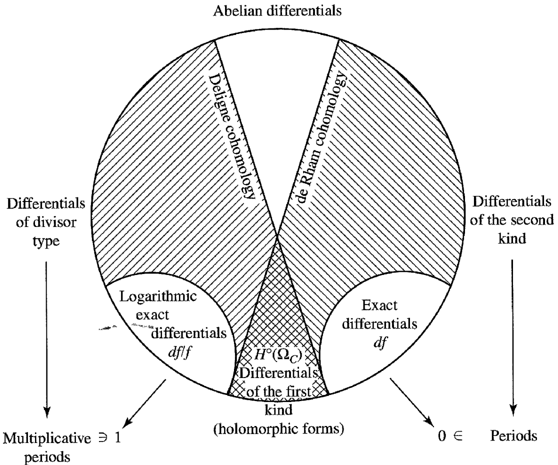
Figure 9.8: Abelian differentials
