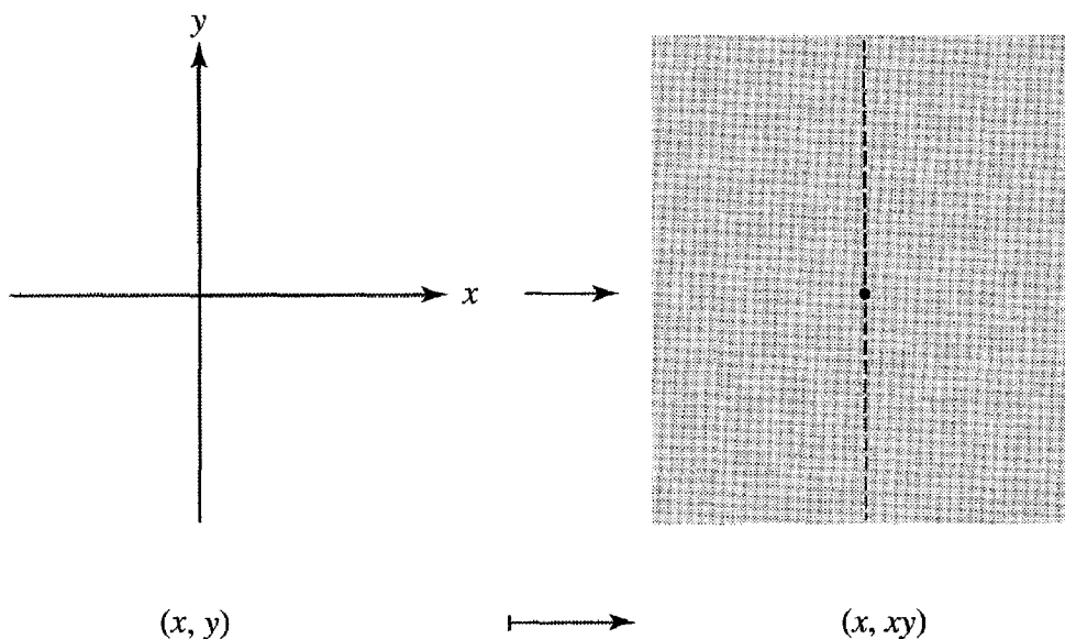
Figure 3.2: The image of a morphism is not necessarily a variety \square
