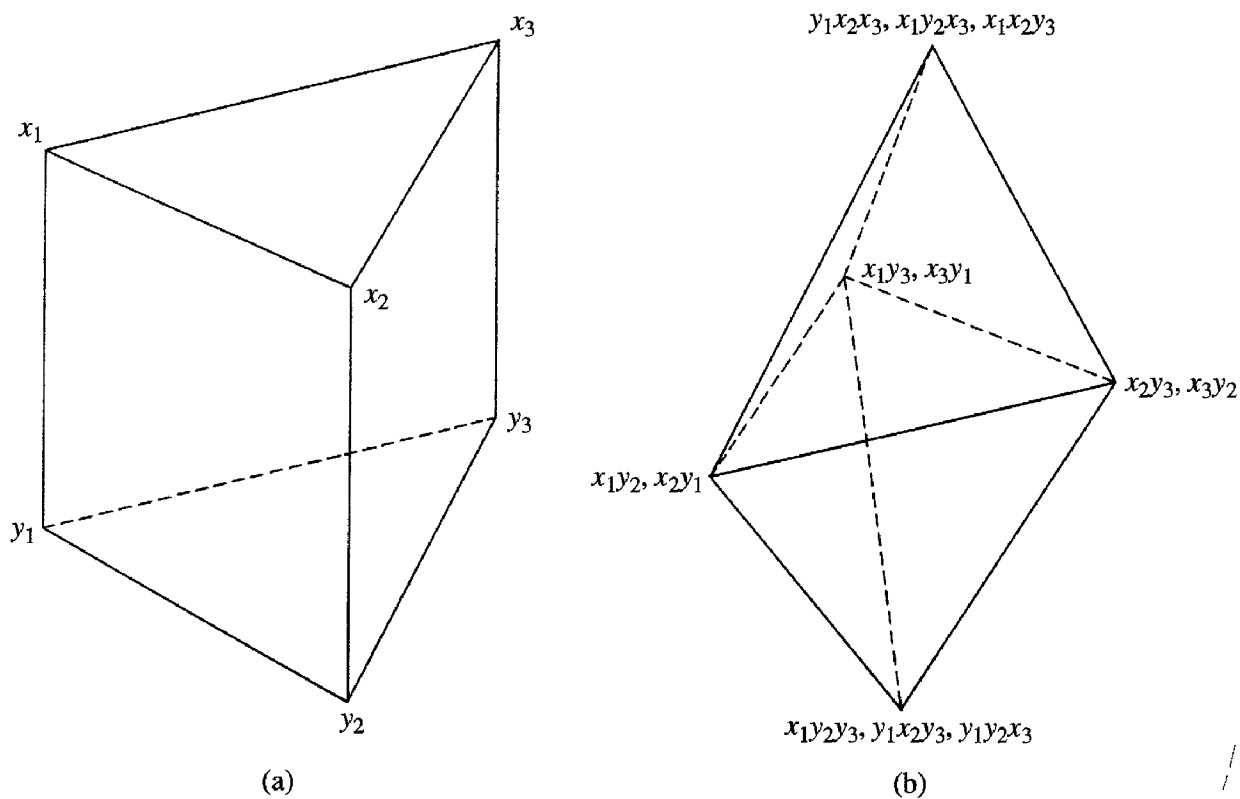
Figure 6.4: Semiinvariants by weight
