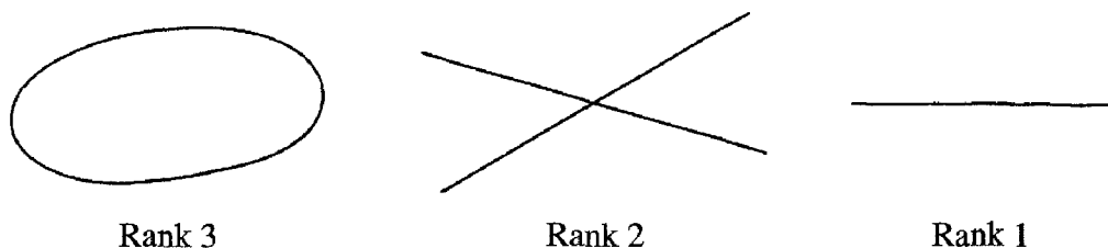
Figure 1.12: Conics over \mathbb{C}
