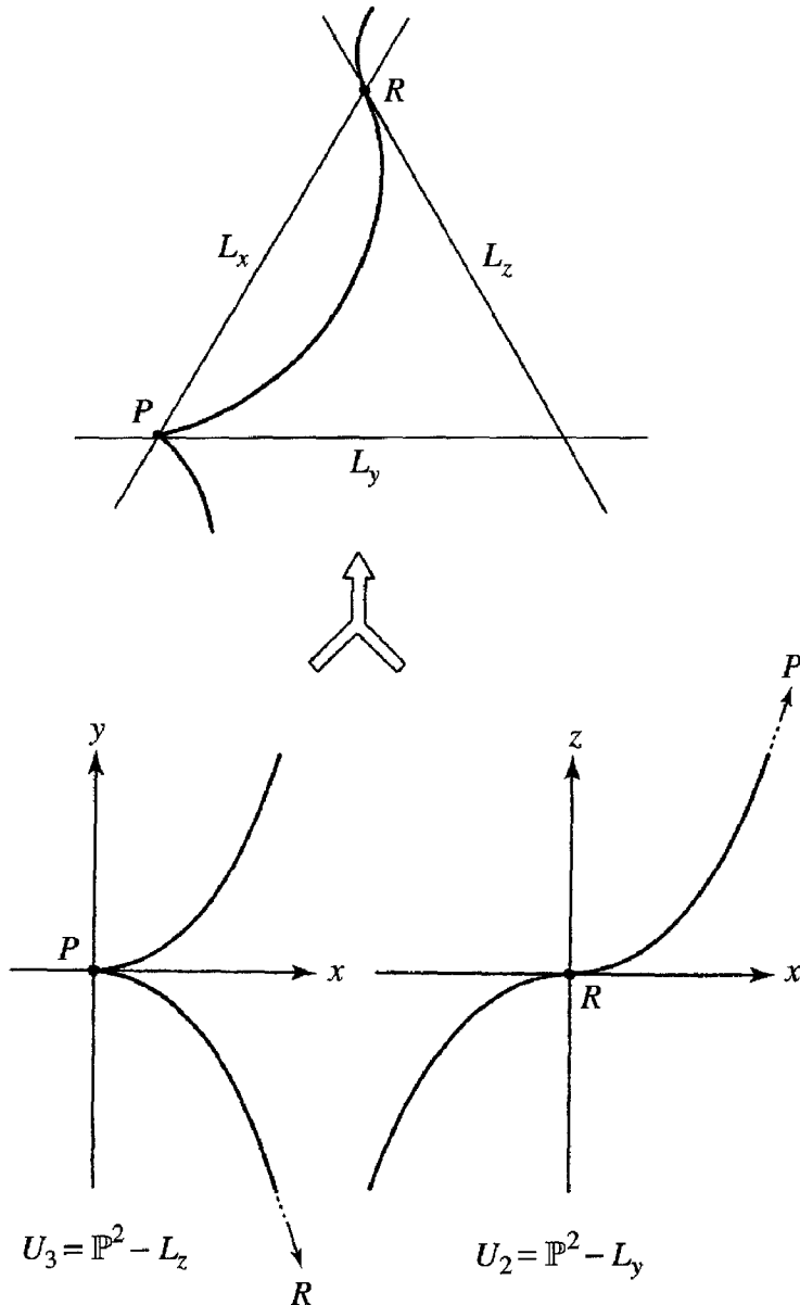
Figure 1.13: The projective curve y^2z - x^3 = 0
