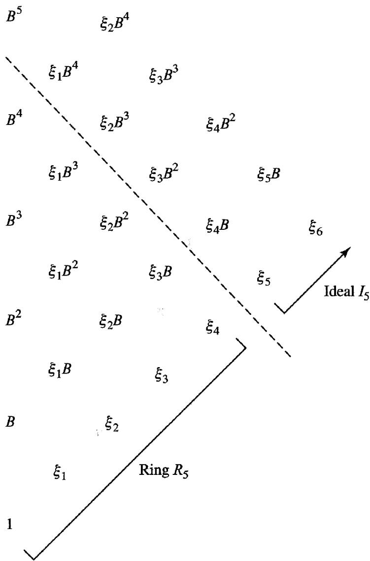
Figure 12.1: The secant ring R_5
