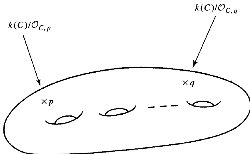
Figure 9.2: The principal part space
