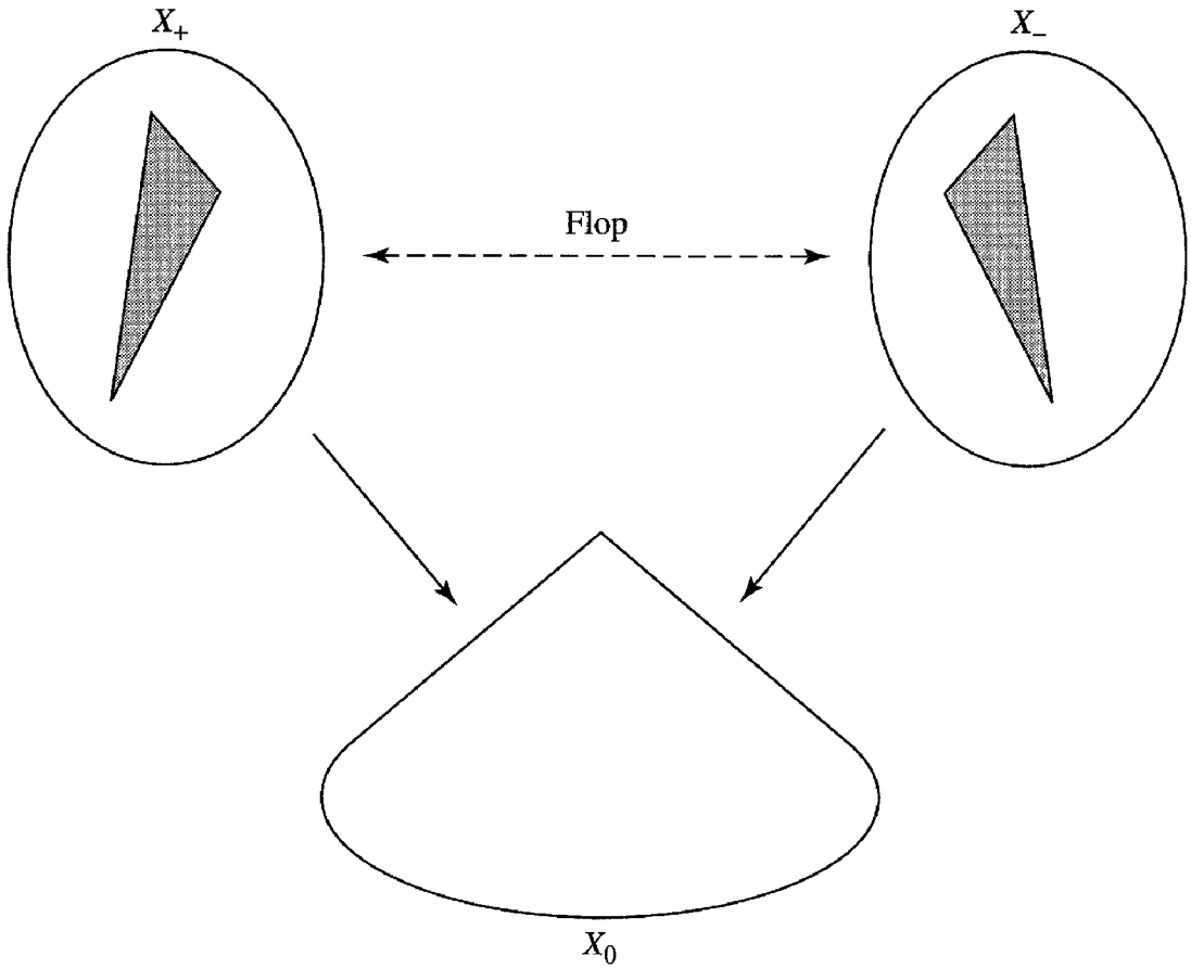
Figure 6.2: A flop
