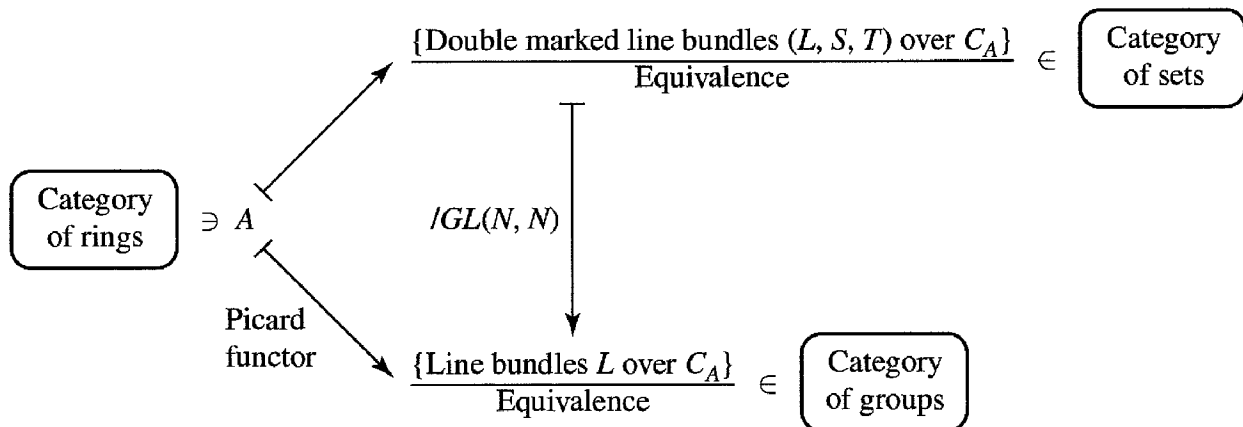
Figure 11.1: The Picard functor
