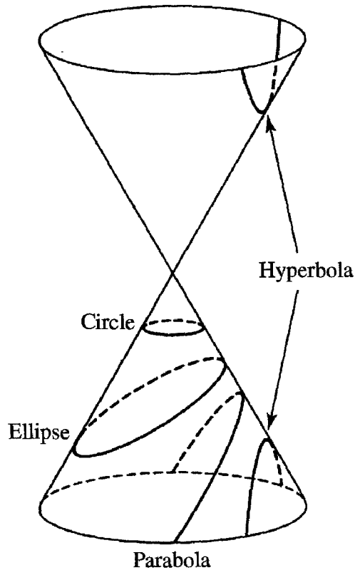
Figure 1.4: Plane sections of a cone
