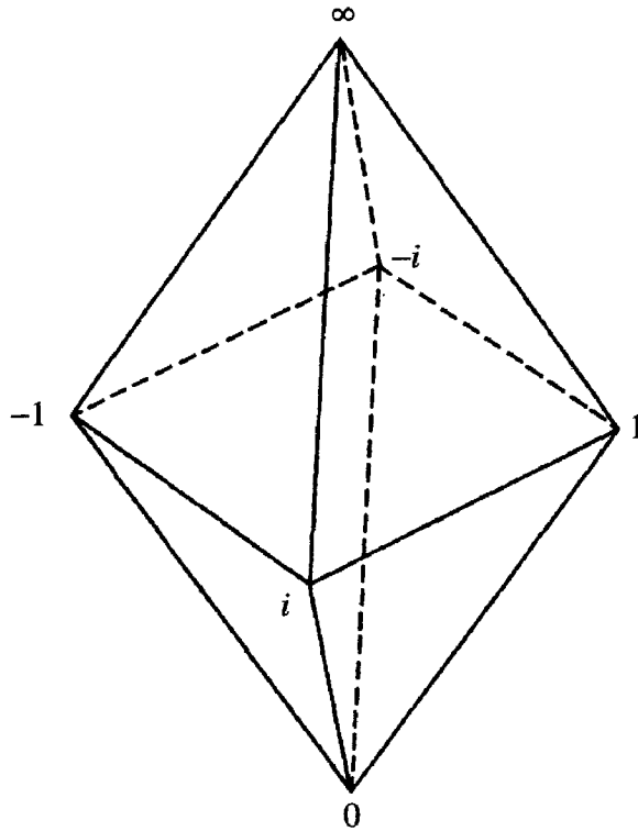
Figure 1.5: The degree 6 invariant and the octahedron
