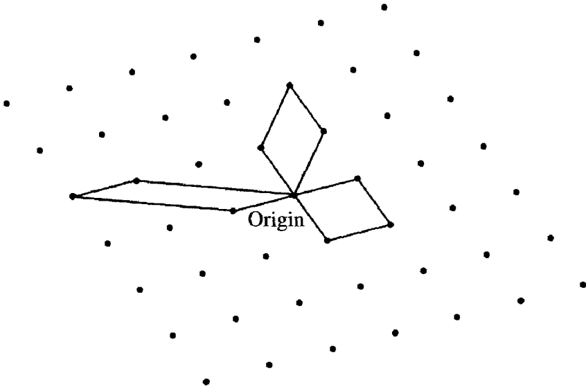
Figure 1.15: Fundamental domains of a lattice.
