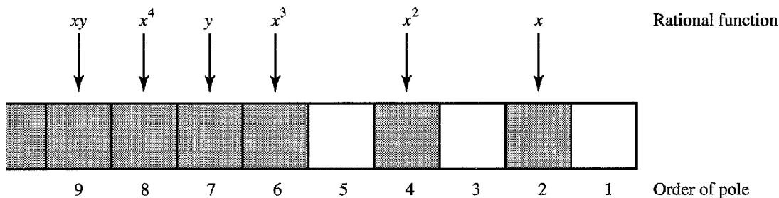
Figure 9.1: The gap values of y^2 = x^7 - 1
