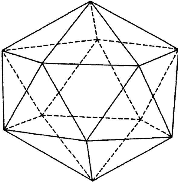
Figure 1.6: The icosahedron
