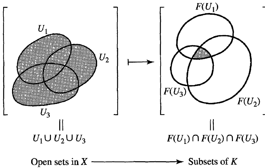
Figure 3.1: An elementary sheaf
