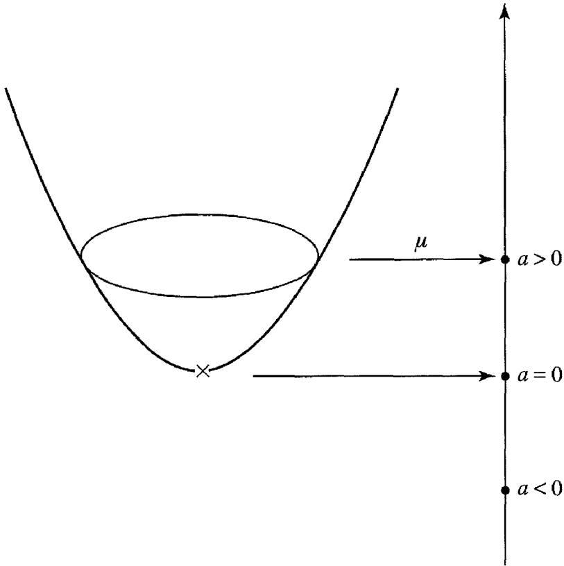
Figure 6.6: The moment map
