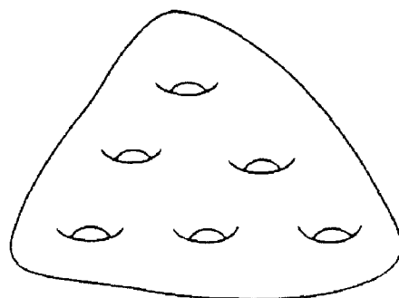
Genus 6
