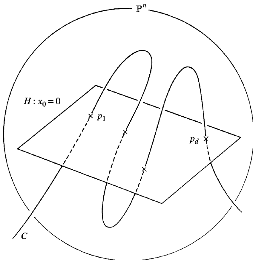
Figure 9.4: A space curve
