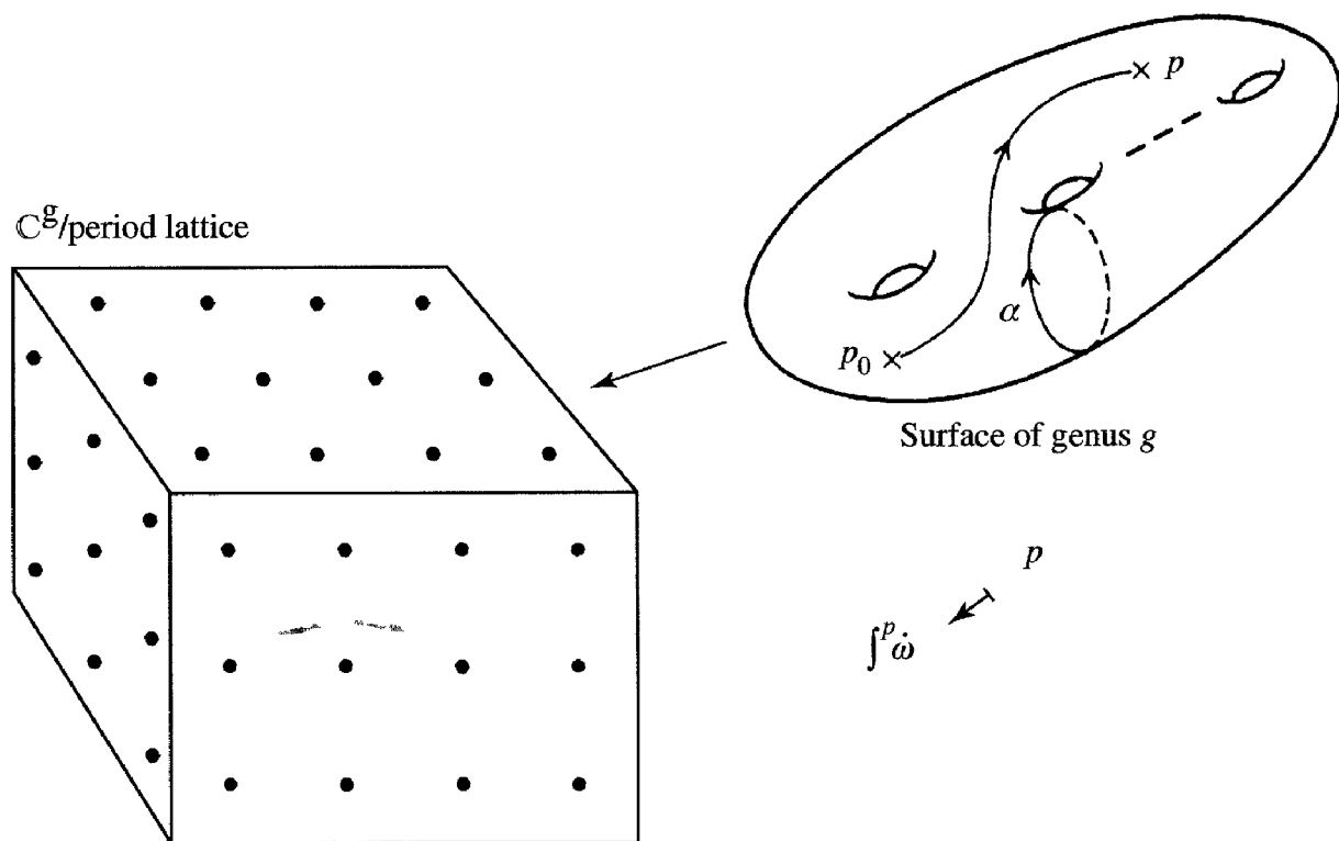
Figure 9.6: The Abel-Jacobi map
