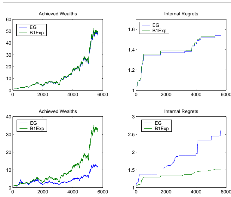
Figure 2. Evolution of both external and internal regrets for the optimal time varying tuning parameter (top) and a 25 times too large one (bottom). Stocks used: Dow Chemical, Coke, GTE, Mei Corp., Gulf, Iroquois, Kin Arc, Amer Brands, Fischbach, Lukens.
