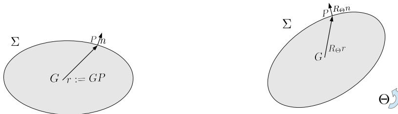
FIGURE 1. On the left, the reference rigid body \Sigma , on the right the rotated rigid body R_\Theta\Sigma
